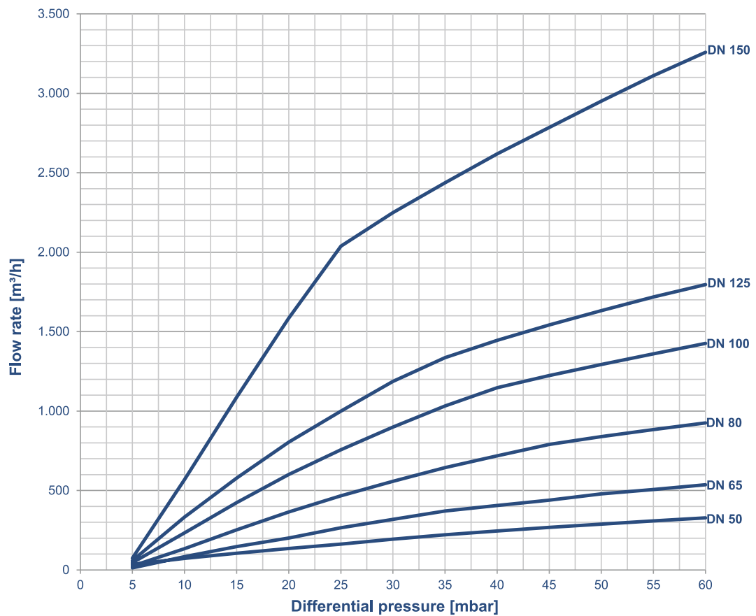
Design diagram Vacuumvalve 6160
