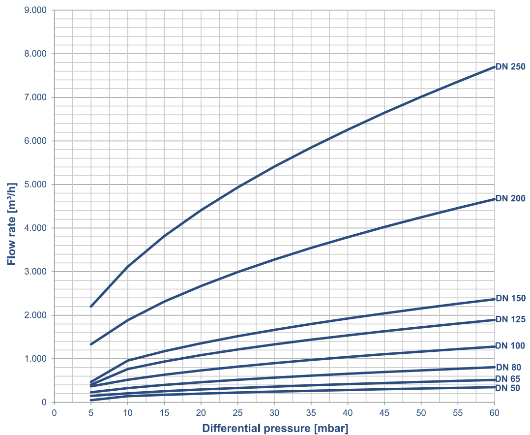
Design diagram Vacuumvalve 6161
